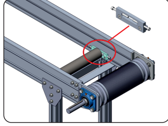
Lower Return Roller Bearing
