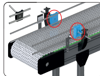
Sensor Mounting Plates
