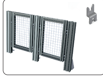
Parallel Connection Part
